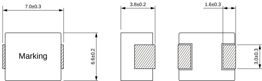
Dimensions: [mm]
