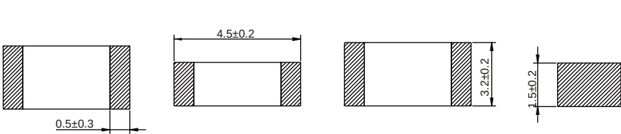
Dimensions: [mm]
